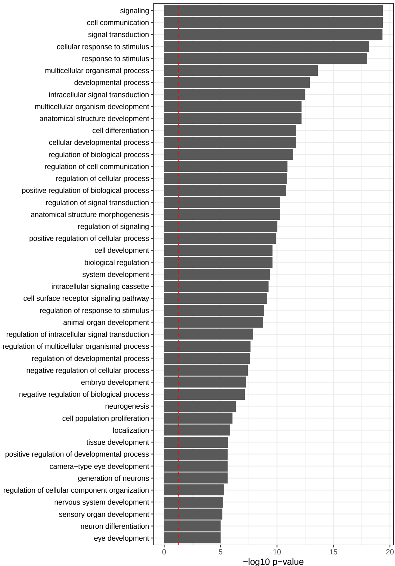
24 hour up DOX_DAR_DEG pairs (within 20kb of TS)
